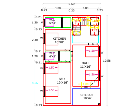
GROUND FLOOR RESIDENTIAL PLAN
