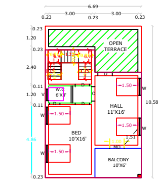
FIRST FLOOR RESIDENTIAL PLAN
