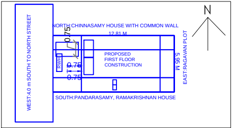
LOCATION PLAN SCALE 1:200
