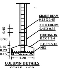
COLUMN DETAILS SCALE - 1:50
