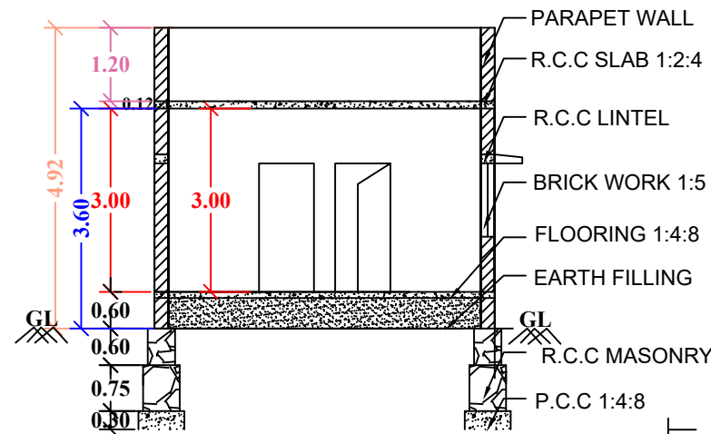
"SECTION "AB"
