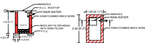
SECTION ON O - P
