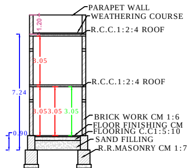
SECTION ON SV
