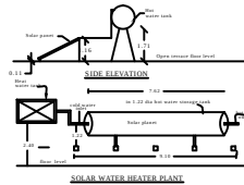
SOLAR WATER HEATER PLANT
