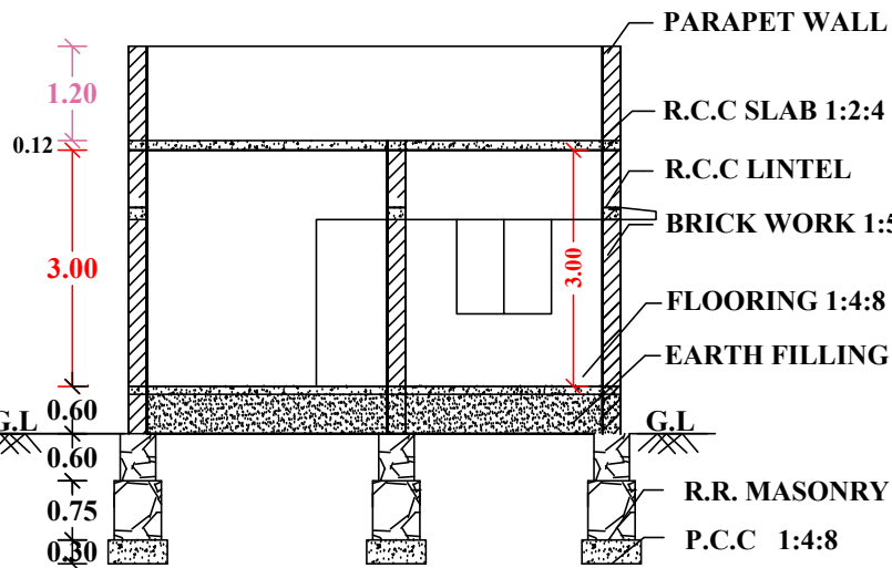
"SECTION "AB"
