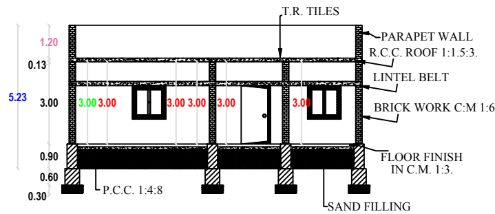
SECTION "AB"
