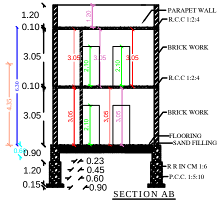
SECTION AB
