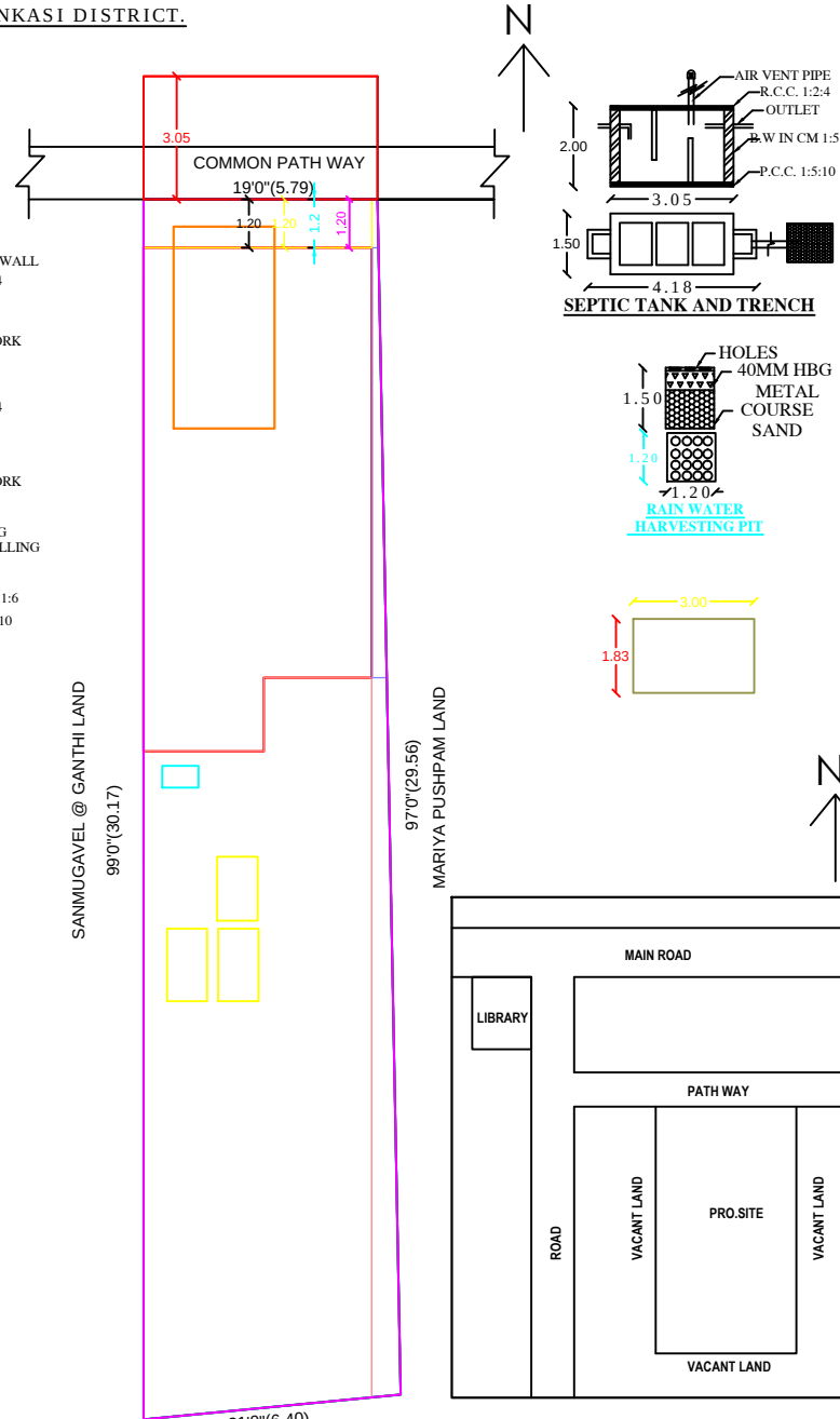
LOCATION PLAN
