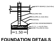
FOUNDATION DETAILS
