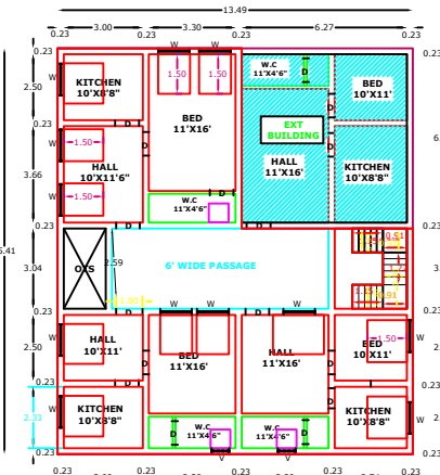
EXT & PRO FIRST FLOOR RESIDENTIAL PLAN
