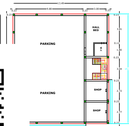
GROUND FLOOR RESIDENTIAL PLAN
