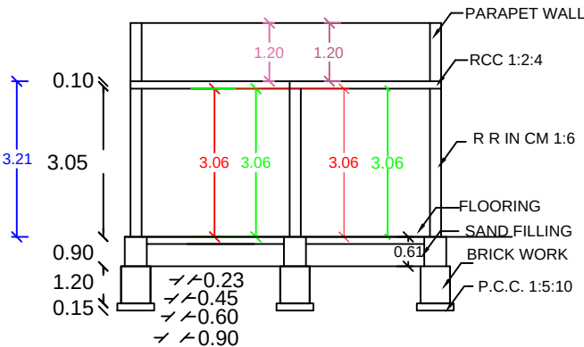
SECTION AB
