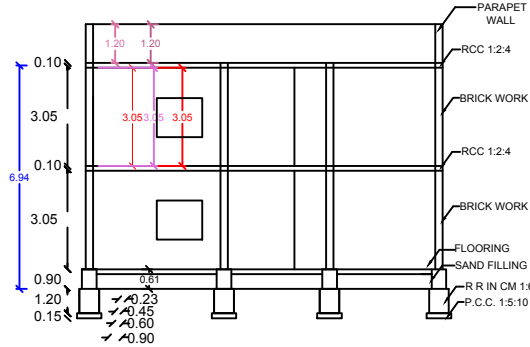
SECTION AB
