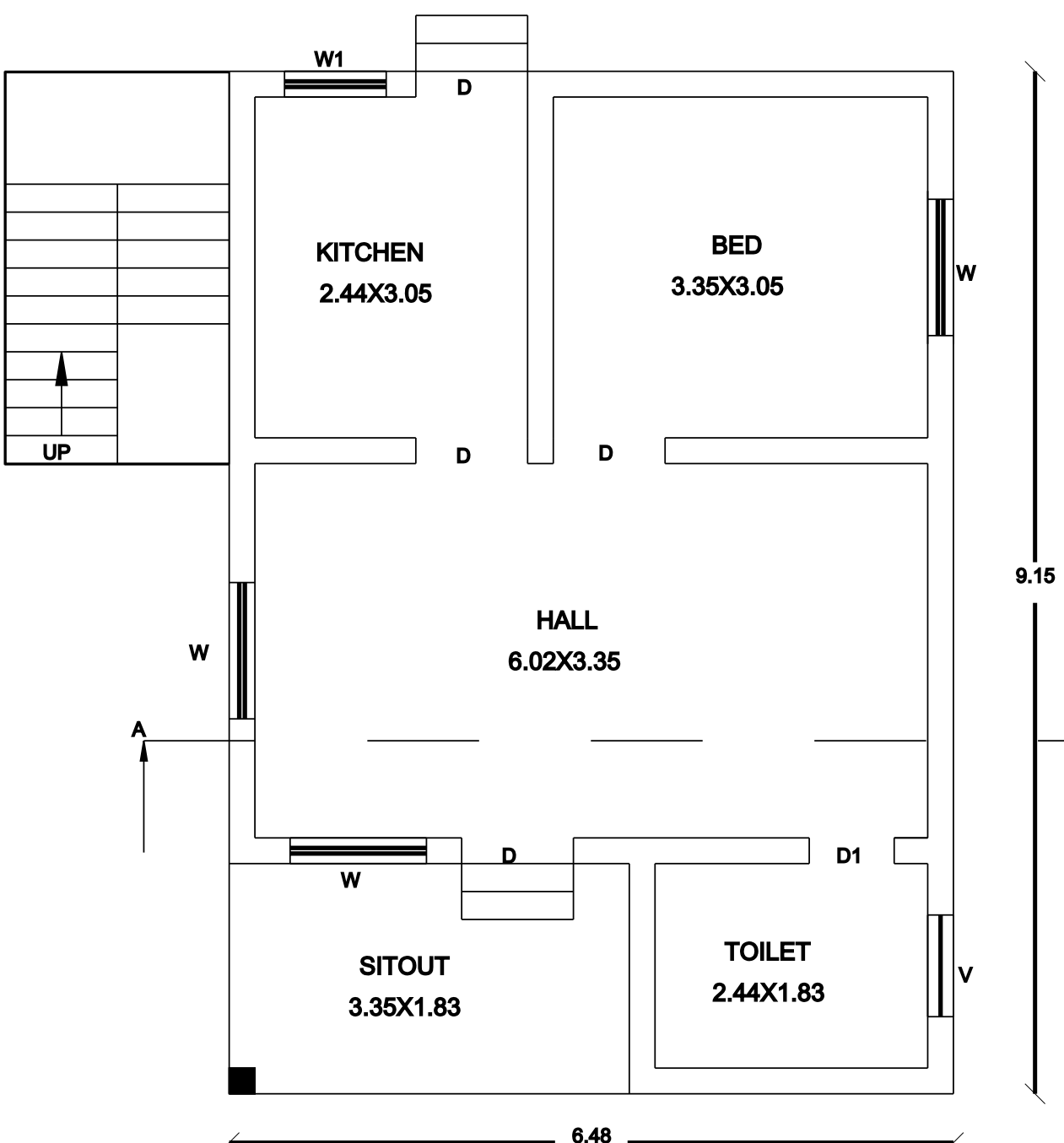
PLAN
