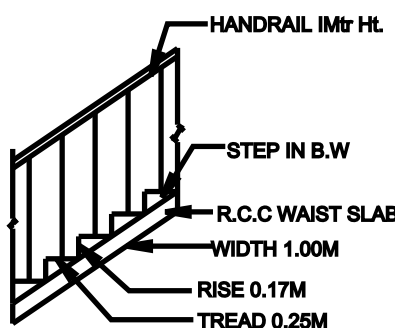
STAIR DETAIL
