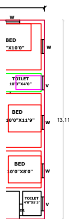
PLAN
