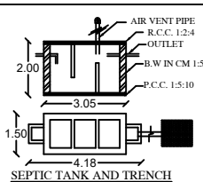
SEPTIC TANK AND TRENCH
