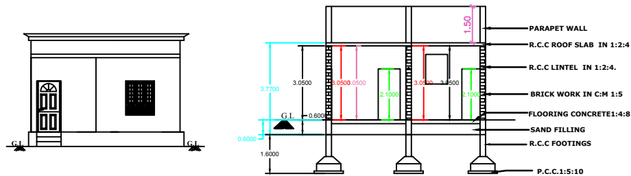
CROSS SECTION ON A-A
