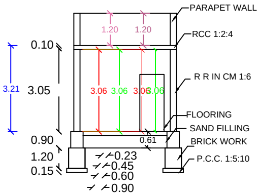
SECTION AB
