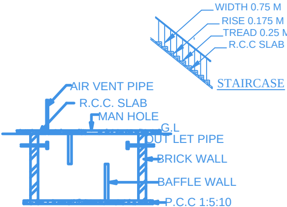
SECTION ON SEP.TANK
