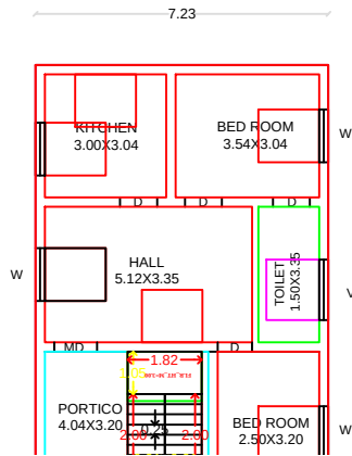
PROPOSED FF PLAN
