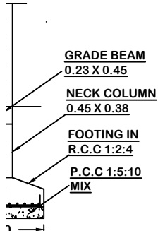
COLUMN DETAILS (SCALE - 1:50)
