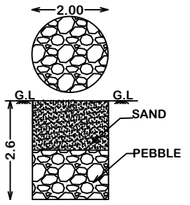
RAINWATER HARVESTING
