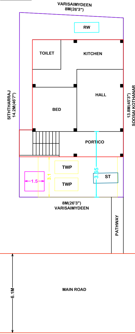
SITE PLAN
