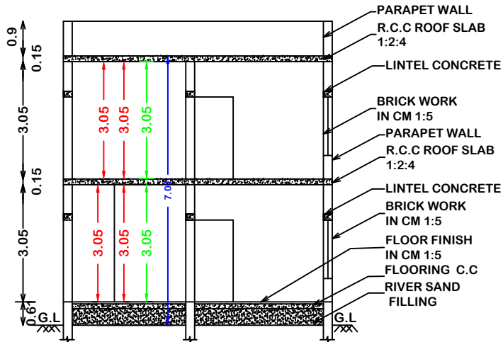
SECTION ON AA1
