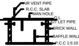
SECTION ON SEP.TANK
