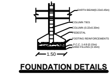
FOUNDATION DETAILS
