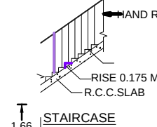
STAIRCASE
