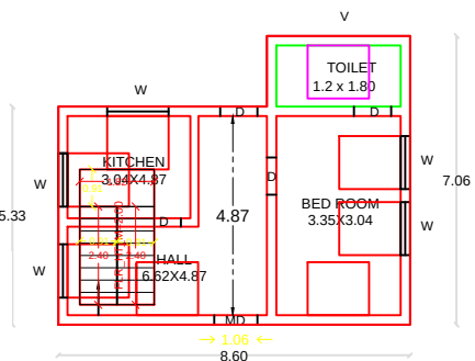
PROPOSED FF PLAN
