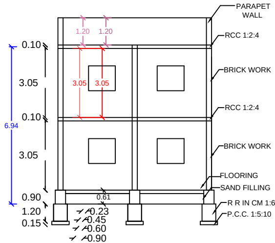
SECTION AB
