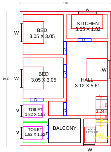
PRO.FIRST FLOOR PLAN
