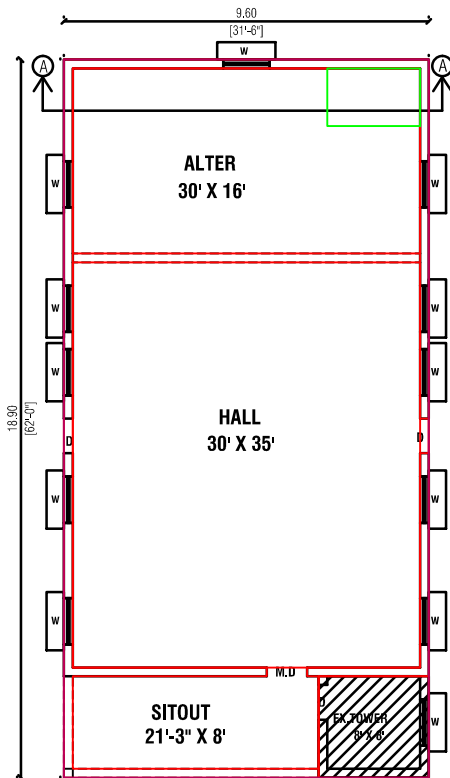
PLAN
