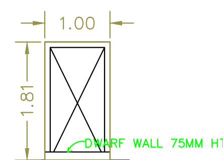
WICKET GATE
