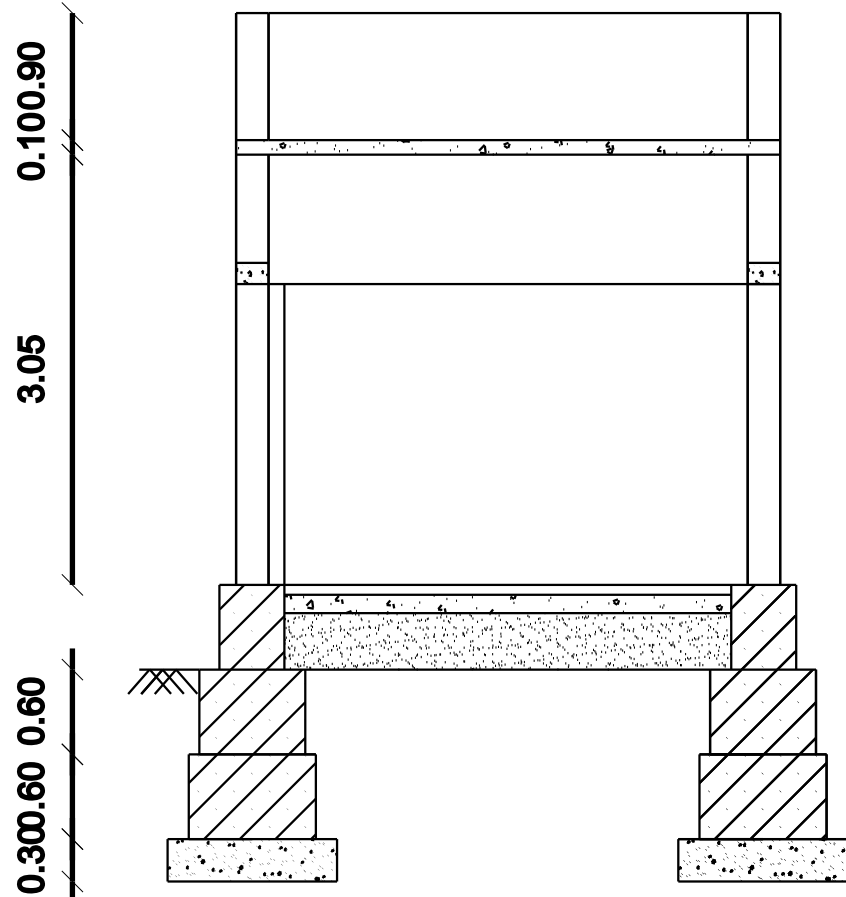
SECTION AA1
