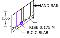
STAIRCASE
