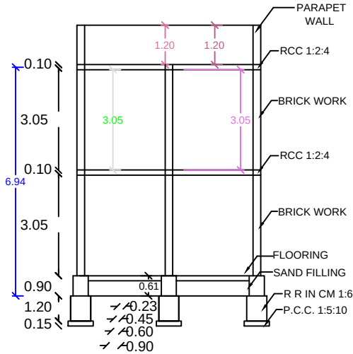
SECTION AB
