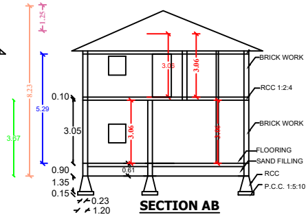
SECTION AB
