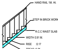
STAIR DETAIL
