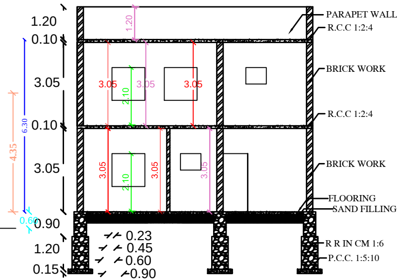
SECTION AB
