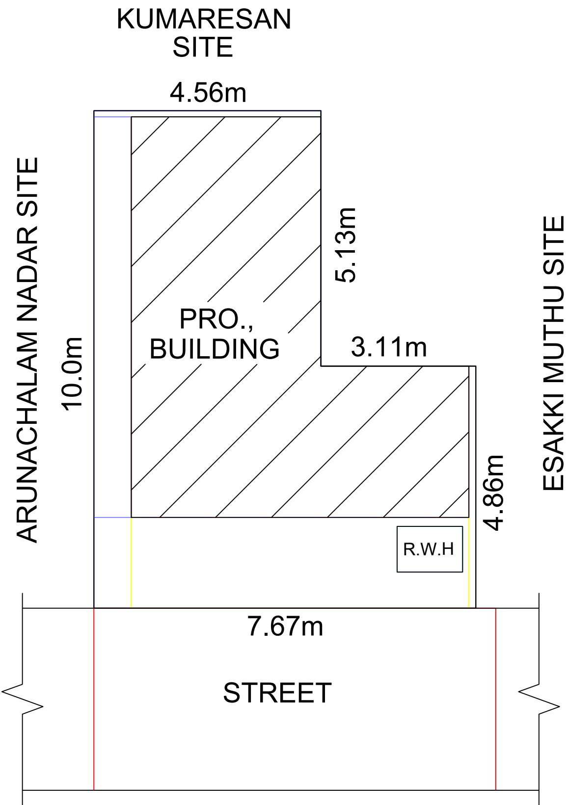
SITE PLAN
