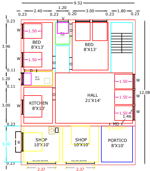
GROUND FLOOR COMMERCIAL CUM RESIDENTIAL PLAN
