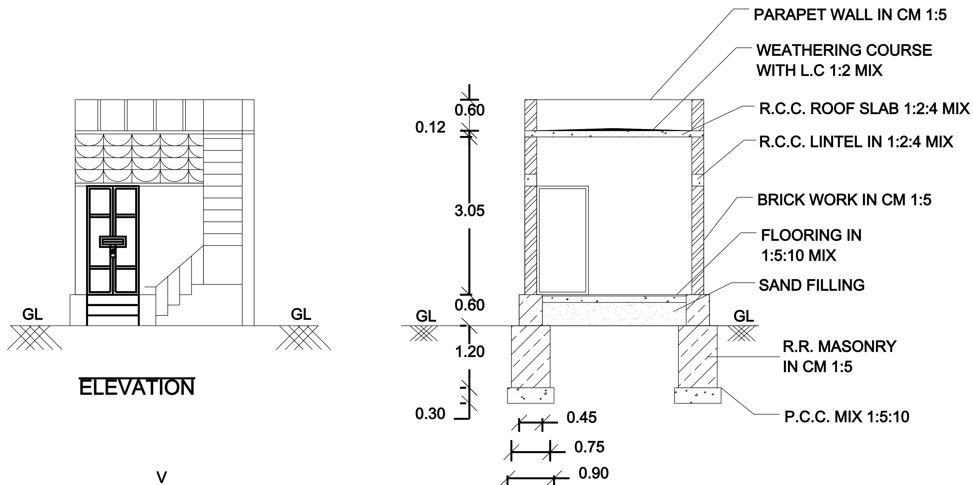
SECTION OF "AB"
