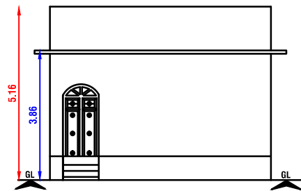
FRONT ELEVATION
