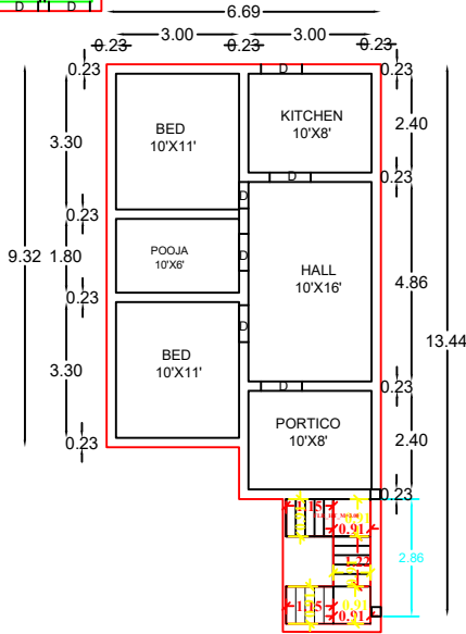
EXT GROUND FLOOR RESIDENTIAL PLAN
