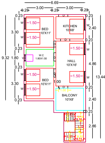
PRO FIRST FLOOR RESIDENTIAL PLAN
