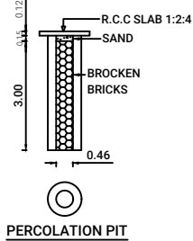
PERCOLATION PIT
