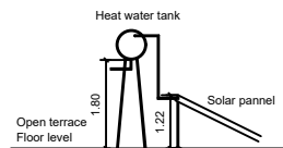
SIDE ELEVATION SOLAR WATER HEATER
