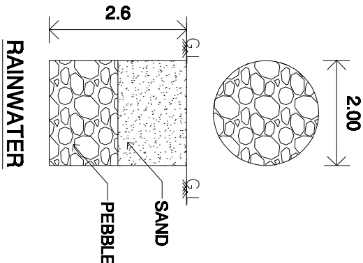
RAINWATER HARVESTING
