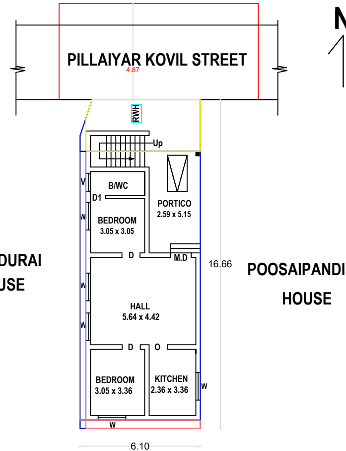
SUBRAMANIAN HOUSE SCALE 1:100
