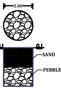
RAINWATER HARVESTING
