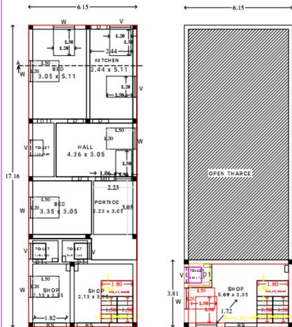
EXG. GROUND FLOOR PLAN
