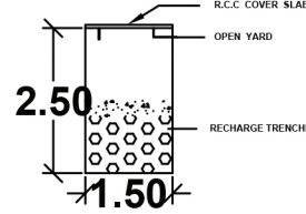
SECTION OF RAINWATER COLLECTING TANK
