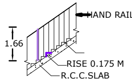
STAIRCASE
