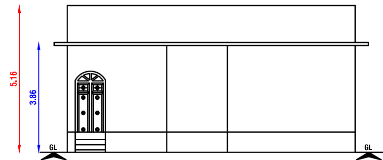
FRONT ELEVATION
