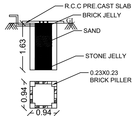
PLAN AND SECTION OF RAINWATER COLLECTION WELL
