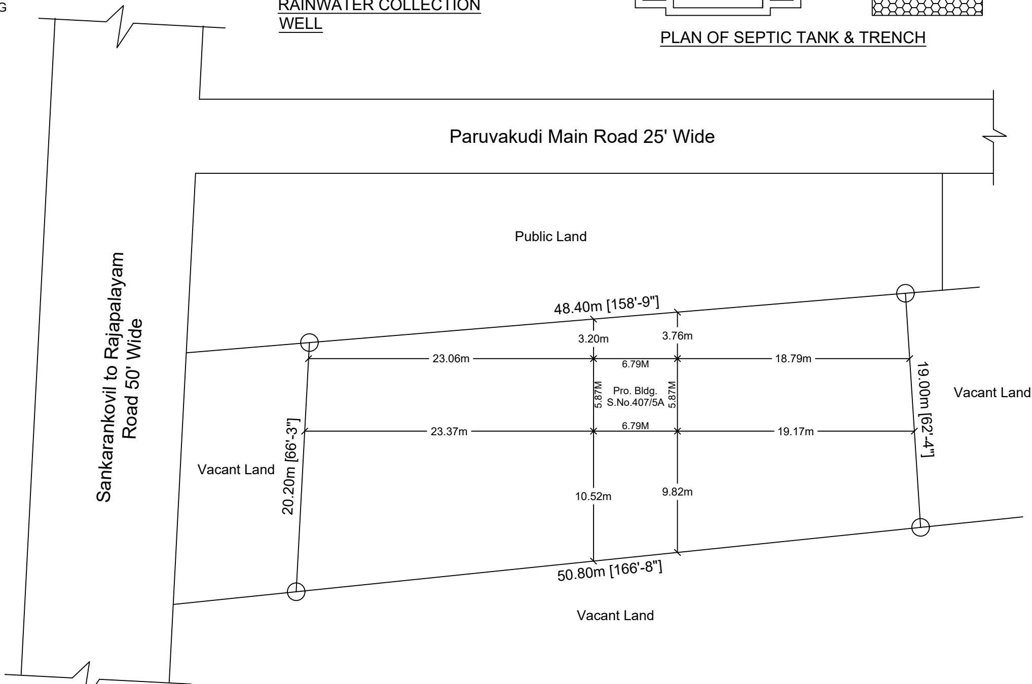
SITE PLAN SCALE = 1:400
