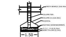
FOUNDATION DETAILS
