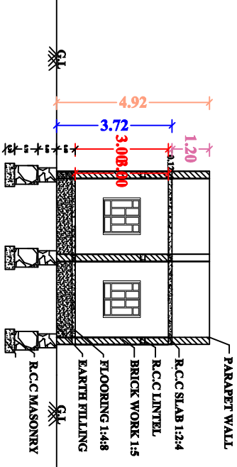
"SECTION "AB"
