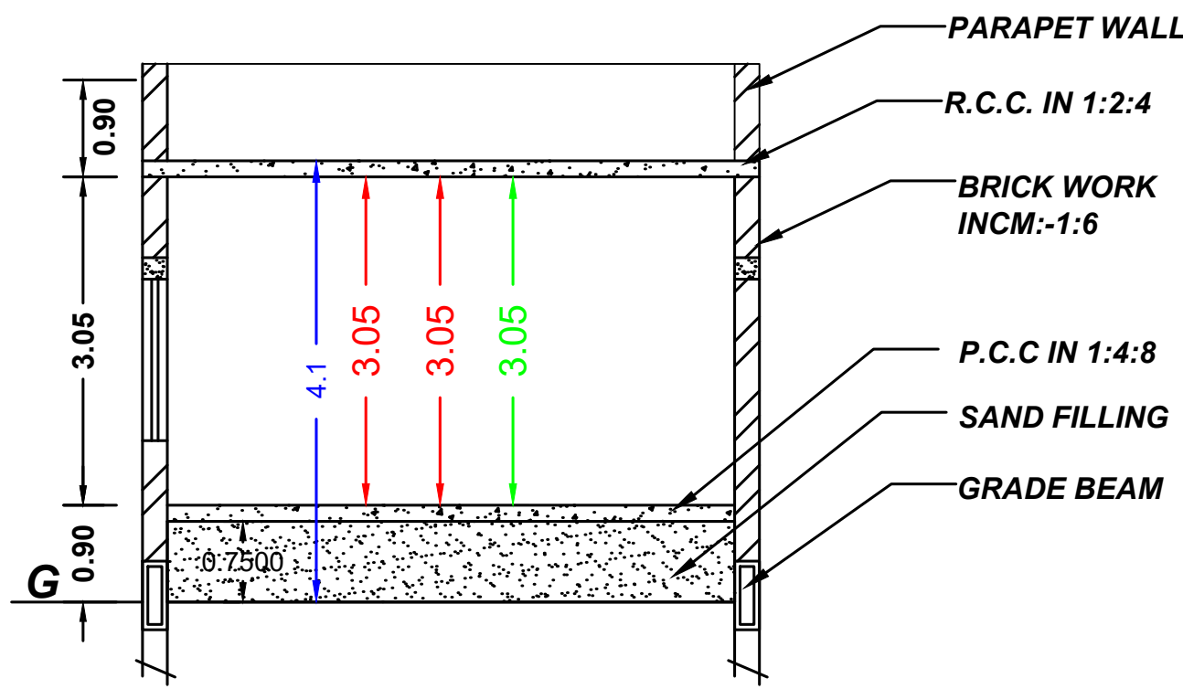
SECTION "AB"
