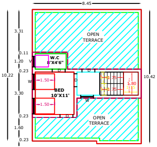
PRO FIRST FLOOR RESIDENTIAL PLAN
