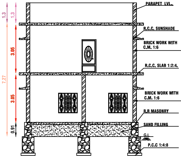
SECTION ON A-A & A'-A'
