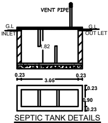
SEPTIC TANK DETAILS
