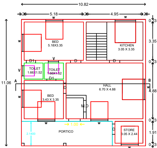
G.FLOOR PLAN
