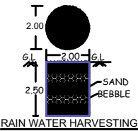
RAIN WATER HARVESTING
